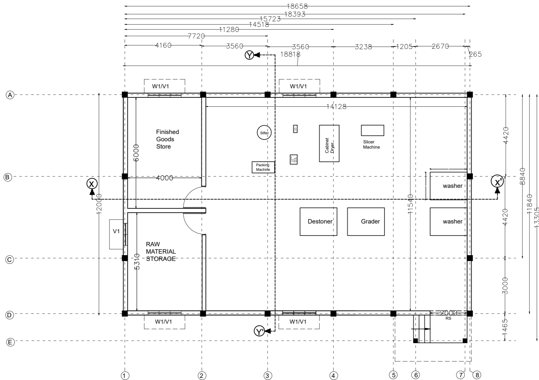
MASALA PROCESSING UNIT BUILD UP AREA - 230 SQM
