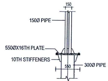
DETAIL A FOR PIPE JOINT
