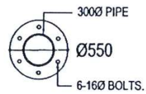
PLAN OF PIPE JOINT
